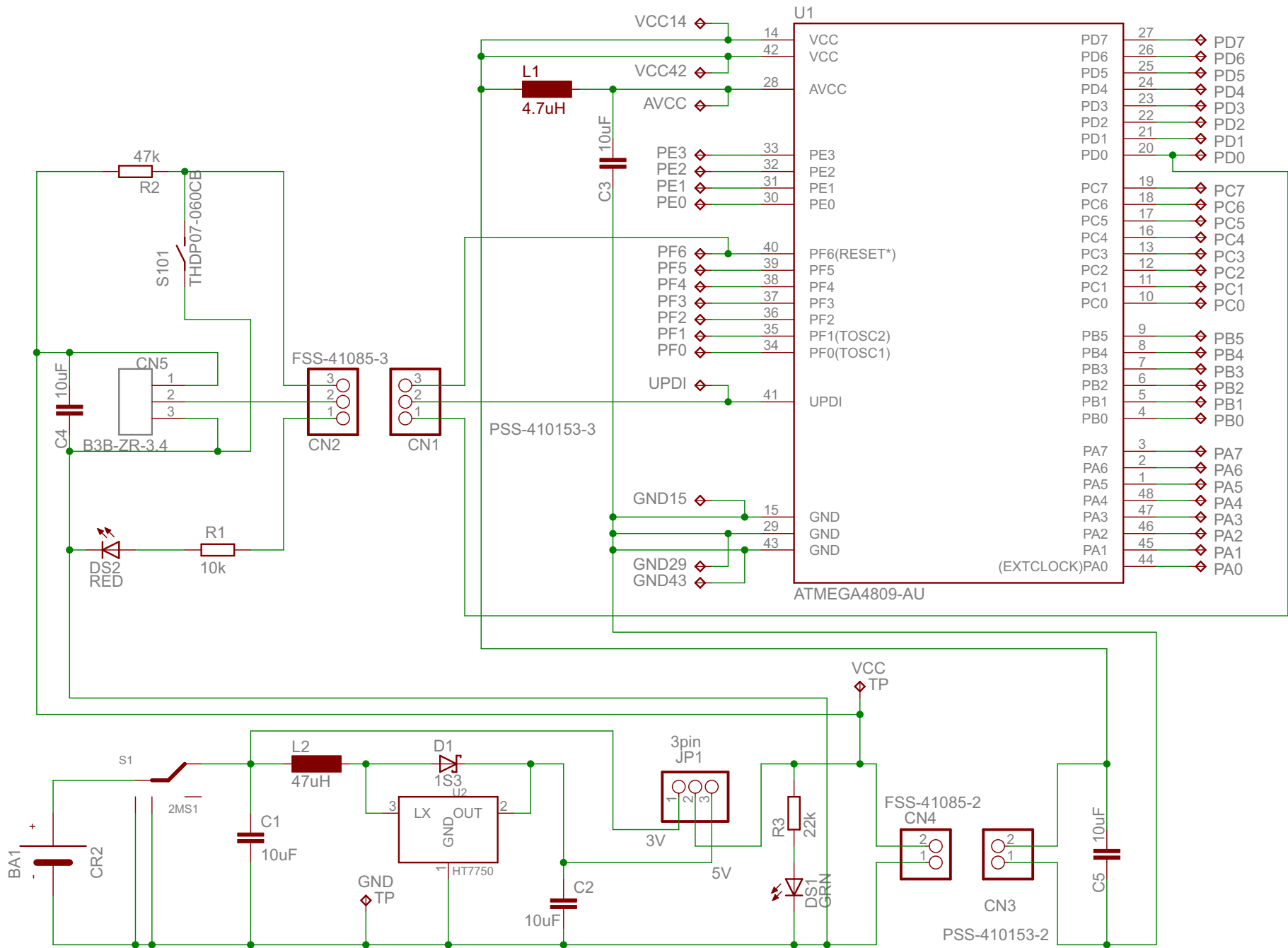
ATmega4809 board cr2 2022/06/09
