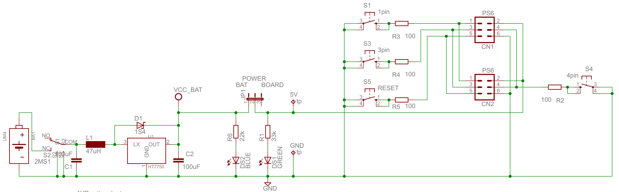
AVR write adaptor 2016/08/16 Taishi
