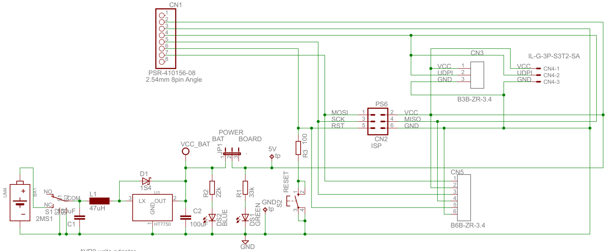
AVR0 write adaptor 2023/06/17 Taishi
