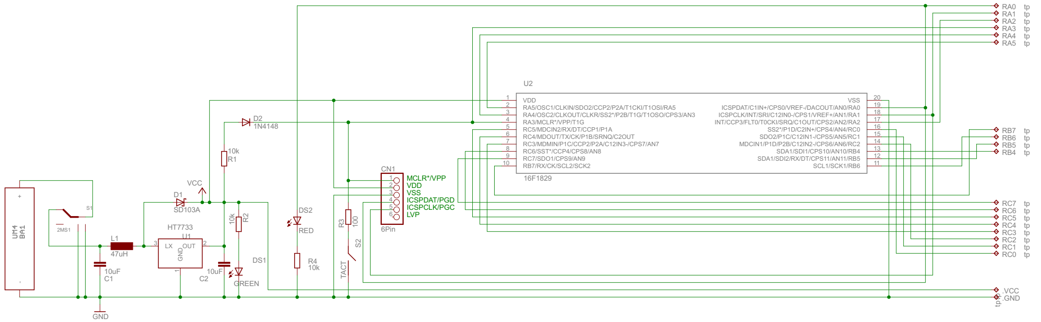
Five_Square_16F1829_LED
