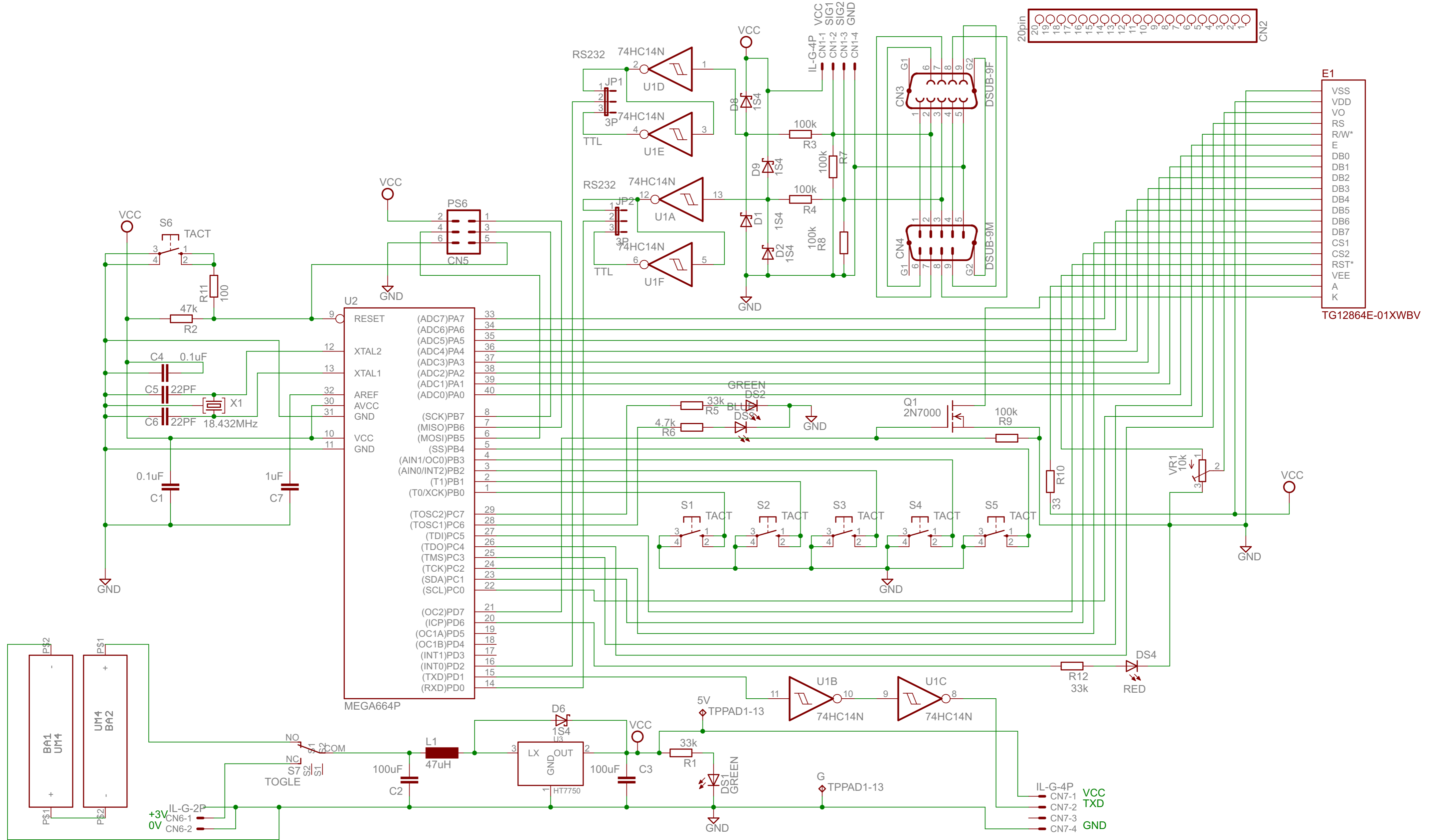
ATmega644 Serial Monitor
