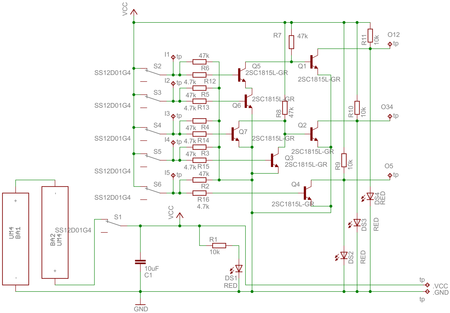
Five_Square_AND_OR_NOT
