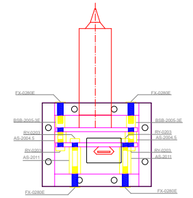
Right Side
