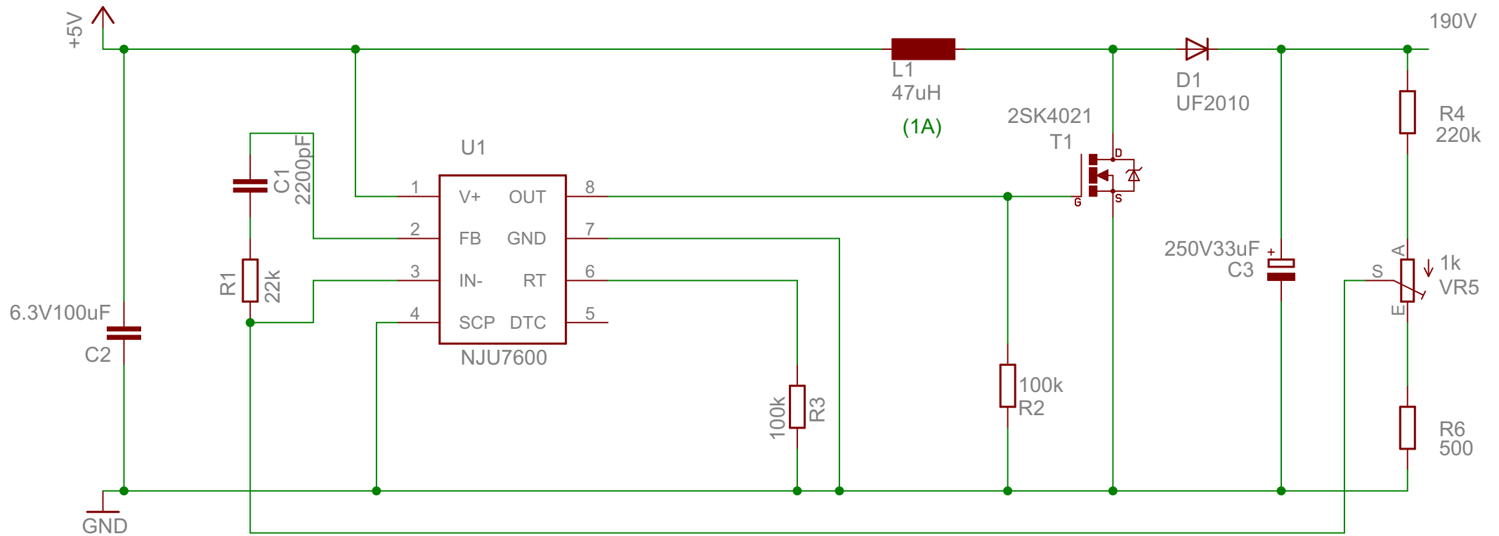
NJU7600 TEST Circuit
