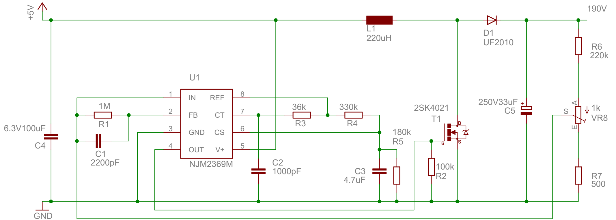
NJM2369 TEST Circuit
